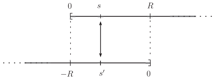
FIGURE 4. Identification -R + s = s'
