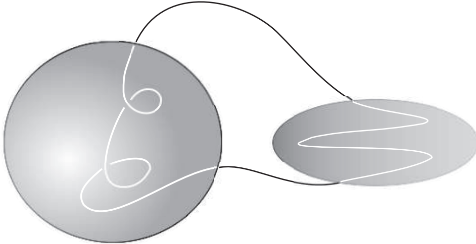
FIGURE 1. This figure shows a M -polyfold, say X , homeomorphic to the space obtained from an open three-ball and an open two-ball connected by two curves having a one-dimensional S^1 -like submanifold. This submanifold could arise as the zero of a transversal section of a strong M -polyfold bundle Y over X , which has varying dimensions. Namely over the three-ball it is two-dimensional, over the two-disk one-dimensional and otherwise trivial. The polyfold theory guarantees natural smooth structures on such solution sets.
