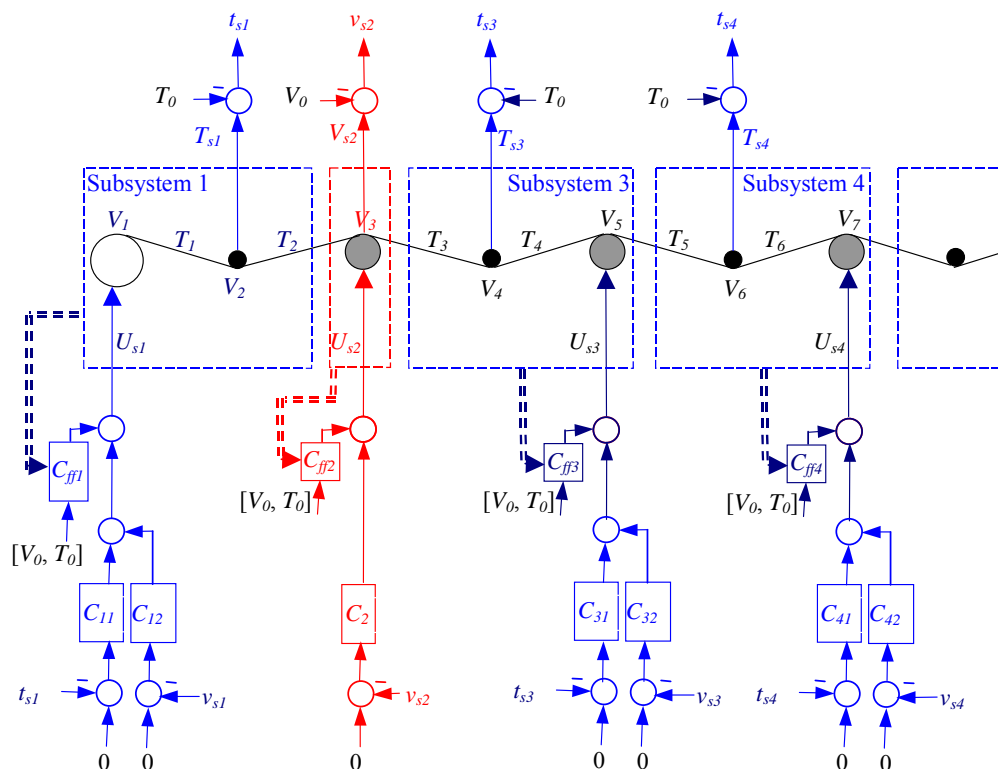
Appendix : decentralized control strategy for a large scale web transport system :
