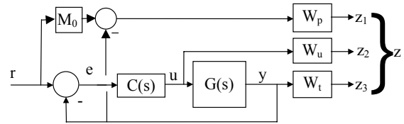
Fig. 3. S/KS/T weighting scheme with model matching for the design of H_\infty control
