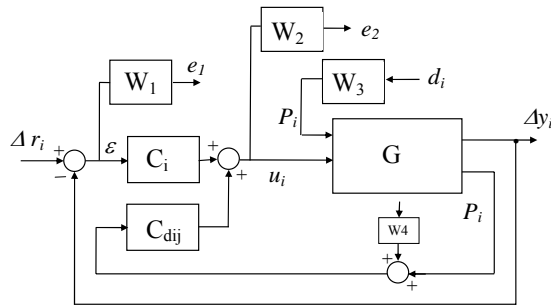
Fig. 7. H_\infty control design with additional measure
