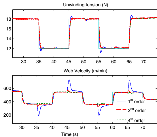
Fig. 5. Simulated web unwinding tension and web velocity for reduced order H_\infty centralized controller
