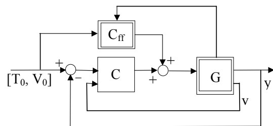
Fig. 6. Control strategy with additive measures and feedforward signals
