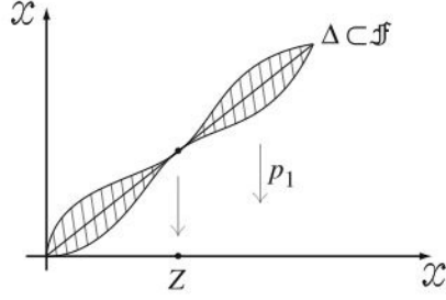
FIGURE 1. Relation afforded by a groupoid with an essential singularity.
